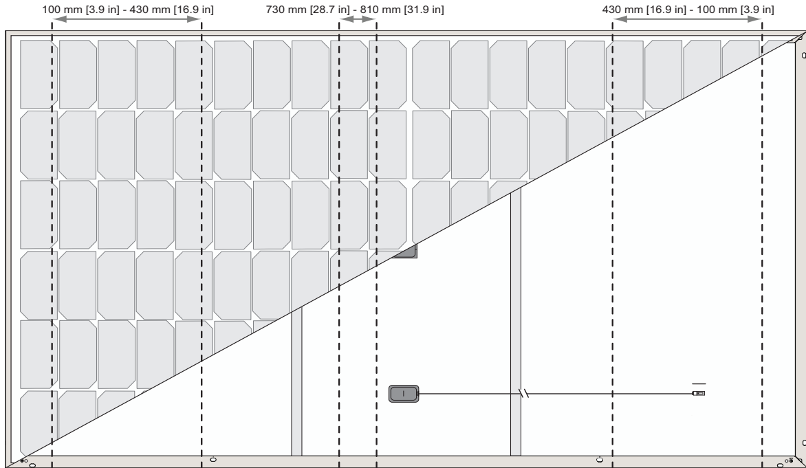
Fig. 15: Six-point mounting configuration clamping zones
